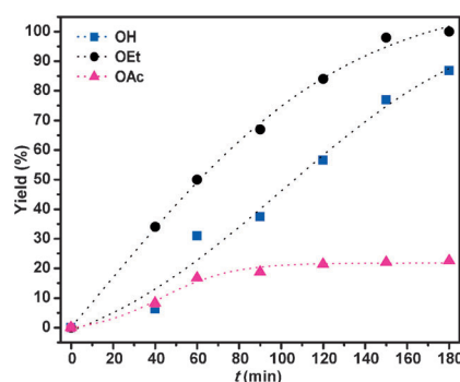
Figure 2. Effect of leaving groups (OH, OEt, and OAc) on the reaction yields. Reaction conditions: 0.50 mmol of substrates, 1.50 mmol of cyclohexanone, 1.0 equiv of pyrrolidine, 6.0 mol% dppe, 2.5 mol% [Pd(η³-allyl)Cl] 2 in CD 3 OD (2 mL).
